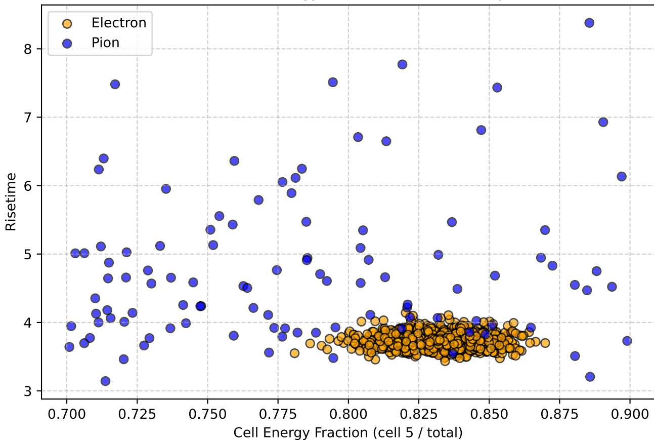
Risetime vs Cell Energy Fraction for 20.0GeV particles
